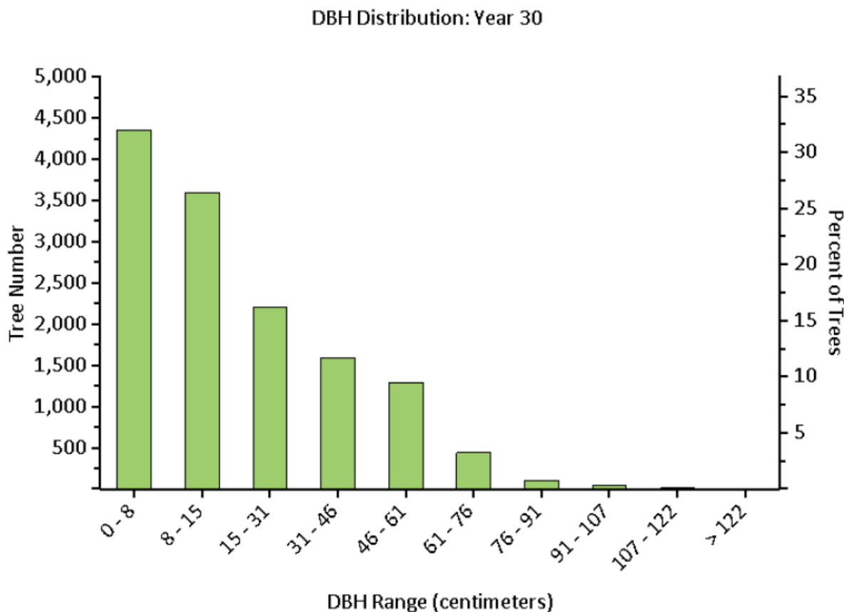
Figure 5. Forecast model results for DBH distribution in the average mortality scenario.
