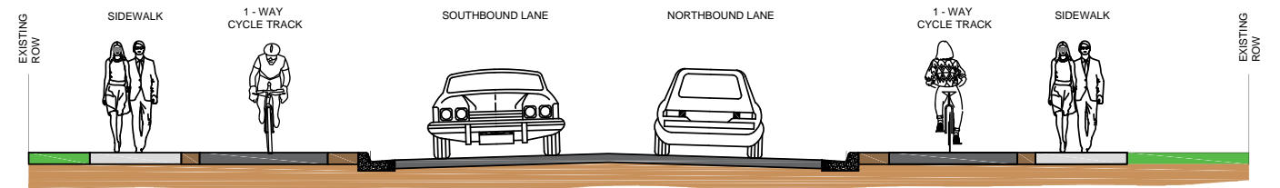
TYPICAL CROSS-SECTION BETWEEN HAWKINS STREET AND DOUGLAS AVENUE
