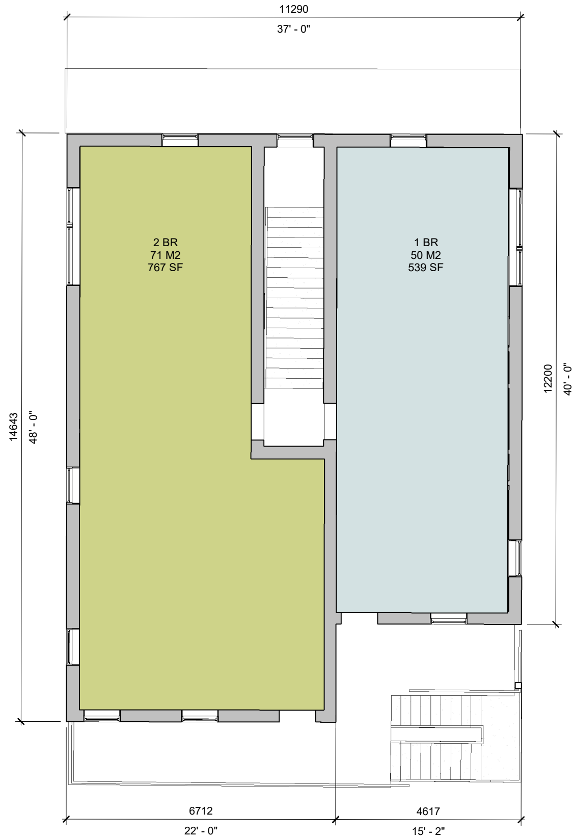
2 LEVEL 2 1/8" = 1'-0"
