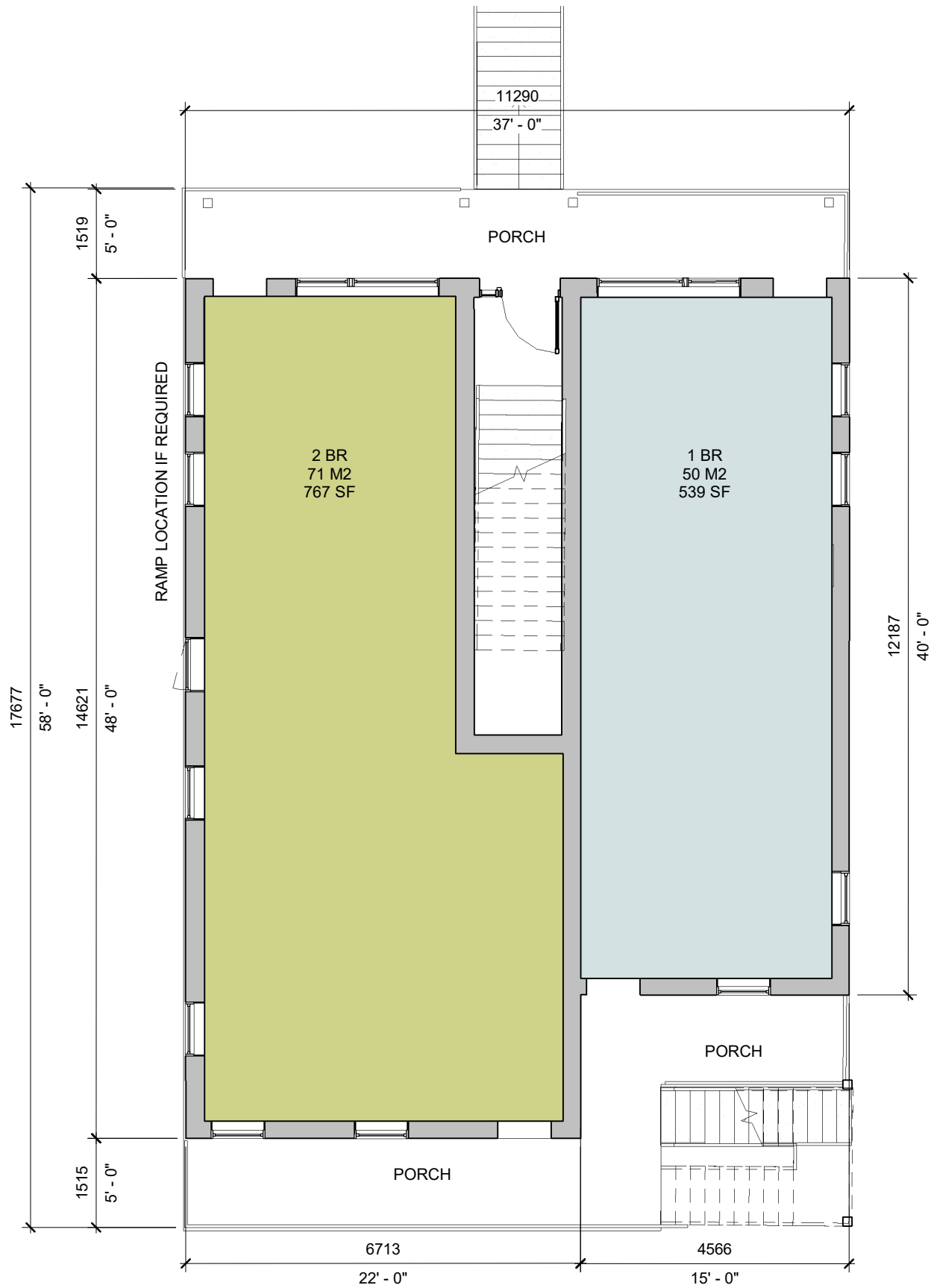
1 LEVEL 1 1/8" = 1'-0"
