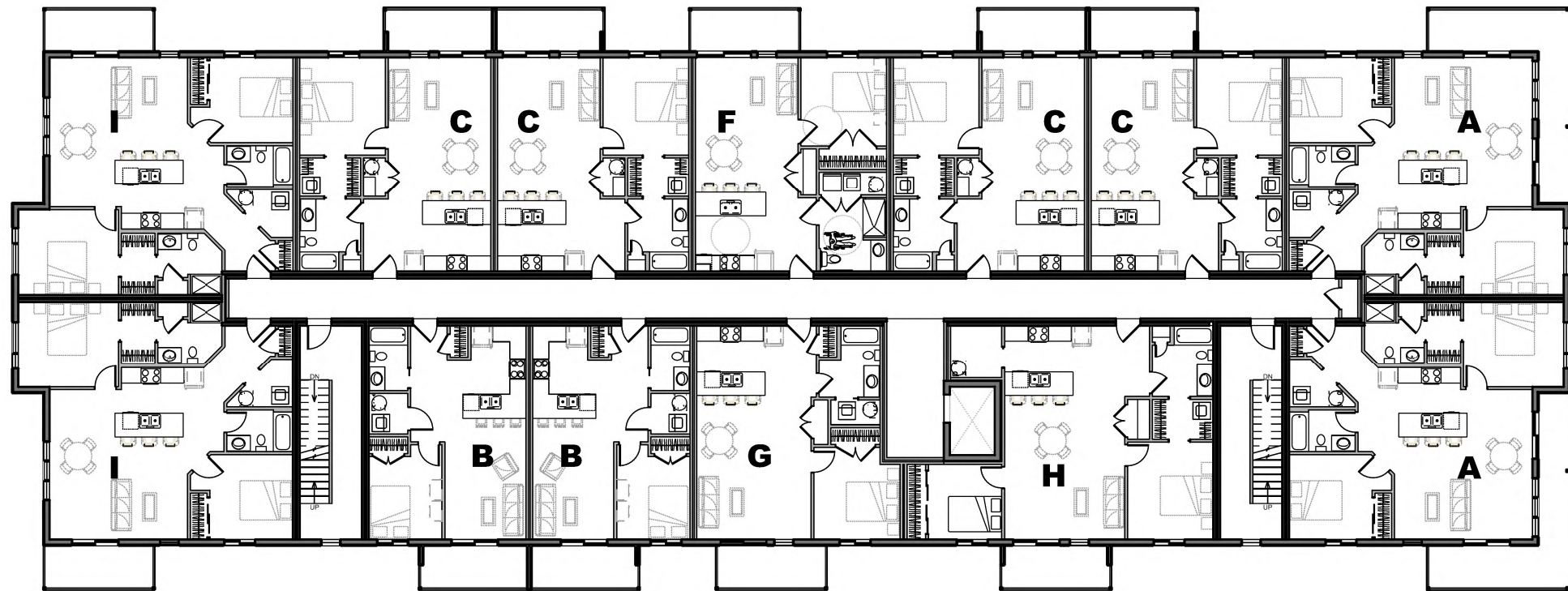
3RD - 5TH FLOOR PLAN
