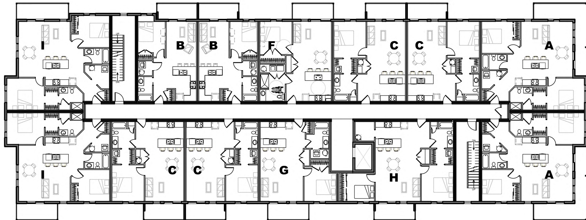
3RD TO 5TH FLOOR PLAN
